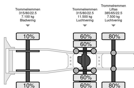
Scania T144.460 V8 DSC1415
