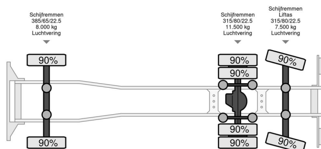
MAN TGX TGX 26.470 - BDF - Retarder - 2021- Steering axle 6x2
