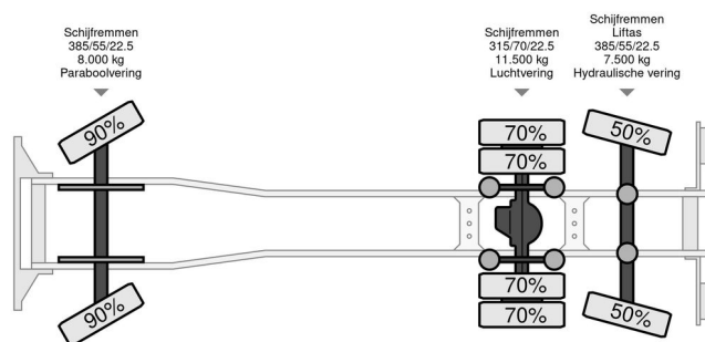
Scania R450 R450 - Retarder - Pig transporter
