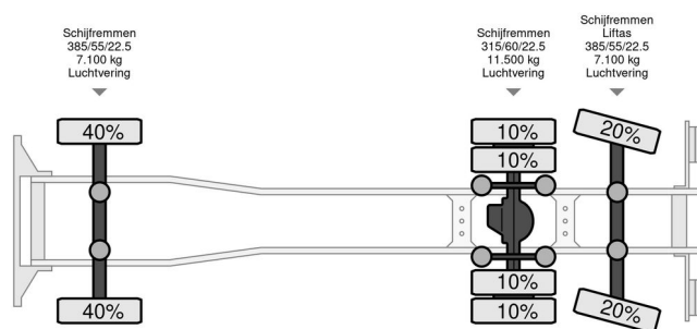
Scania R500 V8 R 500 - Livestock transport - 2006 - Retarder - Geres... 6x2
