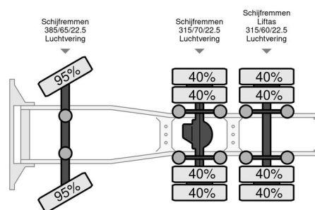
Scania S580 V8
