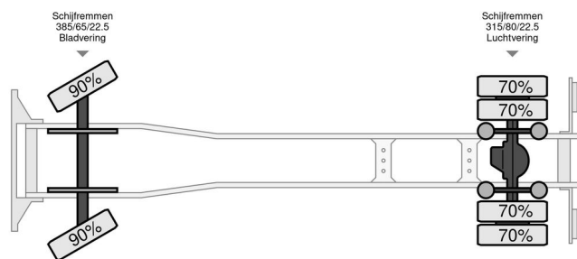
Volvo FH 12-420
