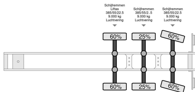
Berdex OS 12.27 Pig transport - 3 levels - steering axle
