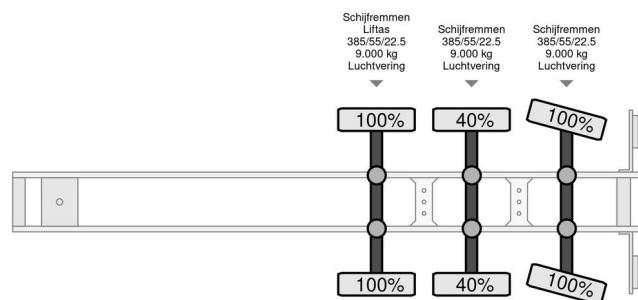
Berdex OS 12.27 - Pig transport - 3 levels - 2007
