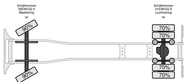
Volvo FH 12.420 FH 12-420 - Platform truck
