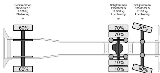
DAF XF 105 105-460
