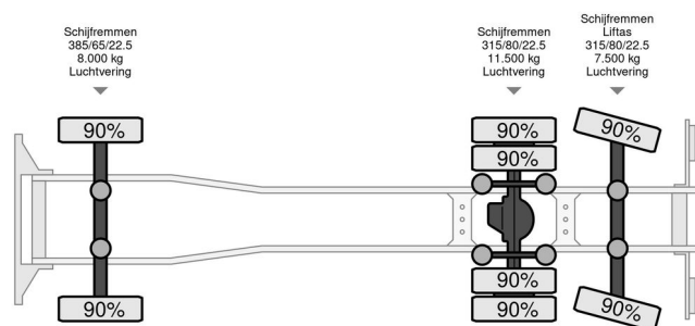
MAN TGX TGX 26.470 - BDF - Retarder - 2021- Steering axle
