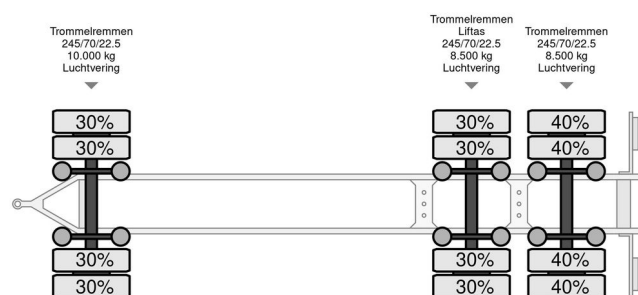
Pezzaioli RBA 31 G - Livestock transport - Cattle transport
