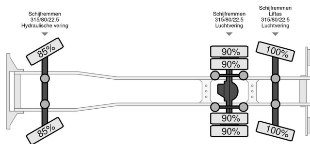
Scania R450 R450- BDF - Steering axle
