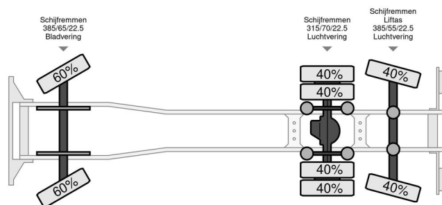
Scania R500 V8 R500LB6X2*4MLA
