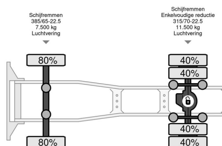
Scania S650 S650 Retarder, Full Air, Full LED, King of the road, PTO N... 4x2 Referentienummer: 13BXD3
