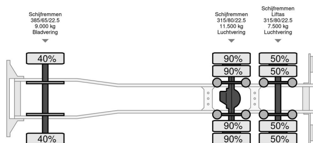
Volvo FH 12.460 FH 12-460 Container systeem - 30 tons
