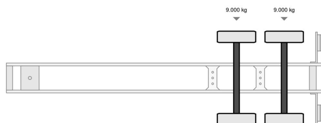
HRD SKFG2Z - Pezzaioli - Livestock transport - 2 Floors - 2 steered axles Referentienummer: OR33ZR
