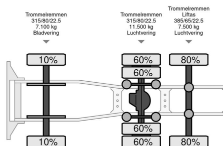
Scania T144.460 V8 DSC1415
