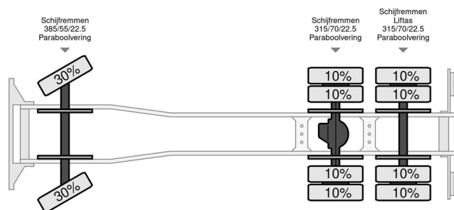
Volvo FH 380
